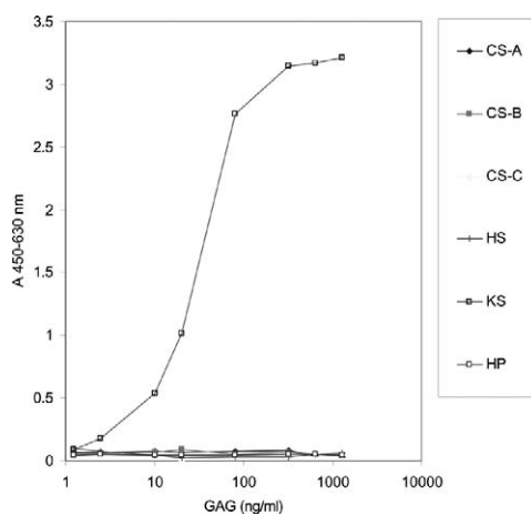
Figure 3 Cross-reactivity of KS-ELISA to KS-related GAGs. The absorbances were plotted against the concentration of each GAG sample. Abbreviations: CS-A, chondroitin sulphate A (Seikagaku # 400658); CS-B, chondroitin sulphate B (Seikagaku # 400660); CS-C, chondroitin sulphate C, (Seikagaku # 400670); HS, heparan sulphate (Seikagaku # 400700); KS, keratan sulphate (Seikagaku # 400610); HP, heparin (Seikagaku # 400610)
